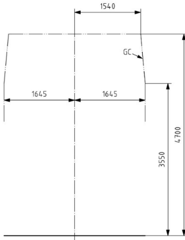
FIGURE 1 KINEMATIC REFERENCE PROFILE GC
