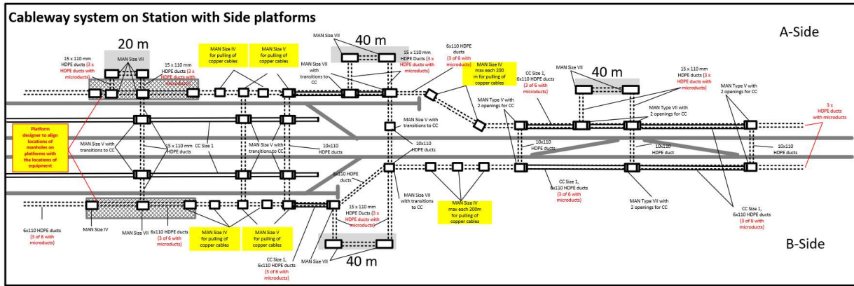
10. CABLEWAYS ON STATION WITH SIDE PLATFORMS
