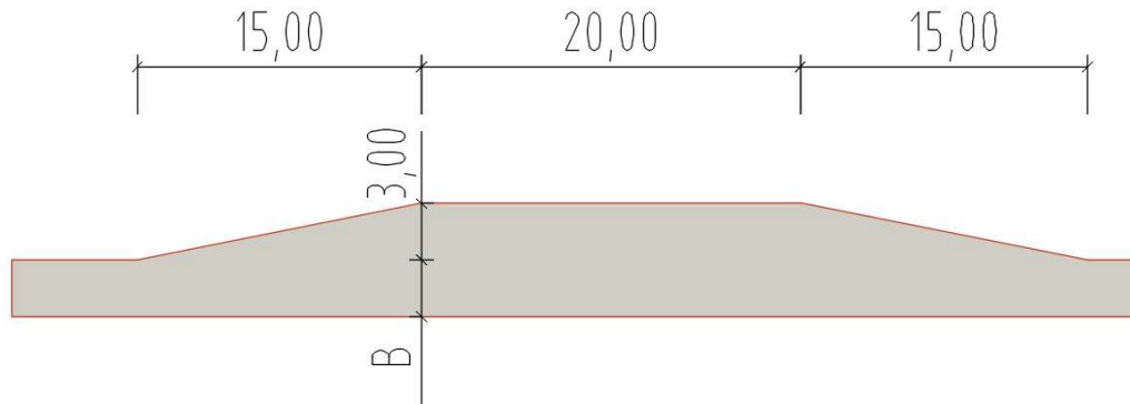
FIGURE 17 PASSING LOOP
