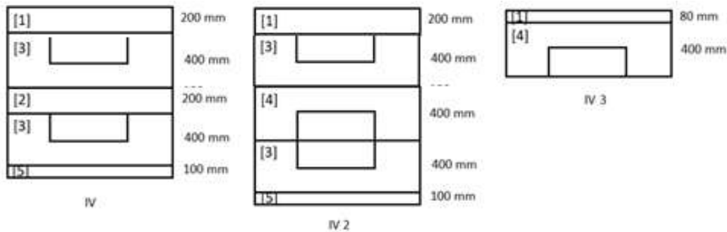
Manholes IV.1, IV.2 and IV.3
