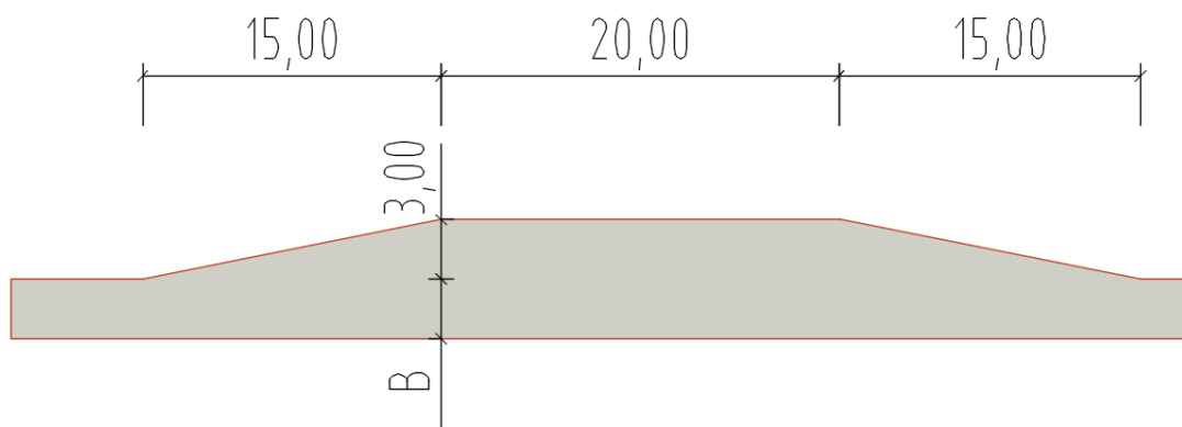
FIGURE 4 PASSING LOOP
