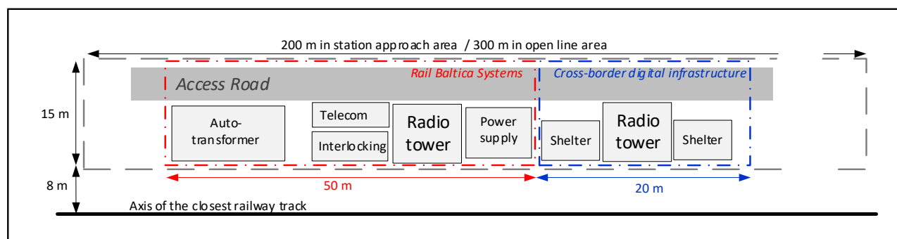
20. LAND PLOT RESERVATION AREA AT SYSTEM EQUIPMENT LOCATIONS
