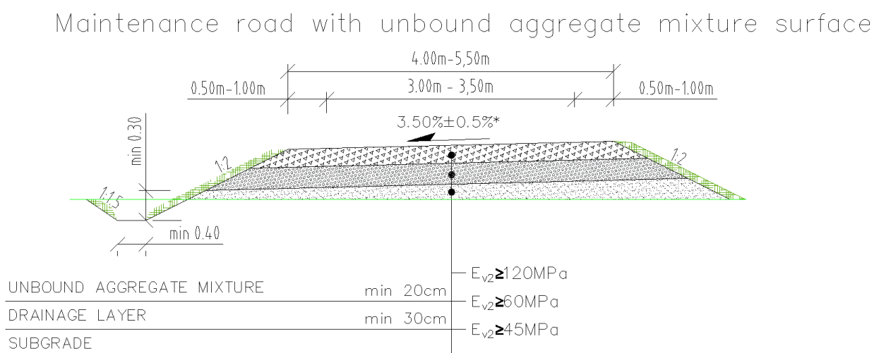
FIGURE 7 TYPICAL MAINTENANCE ROAD CROSS SECTION WITH UNBOUND AGGREGATE MIXTURE SURFACE
