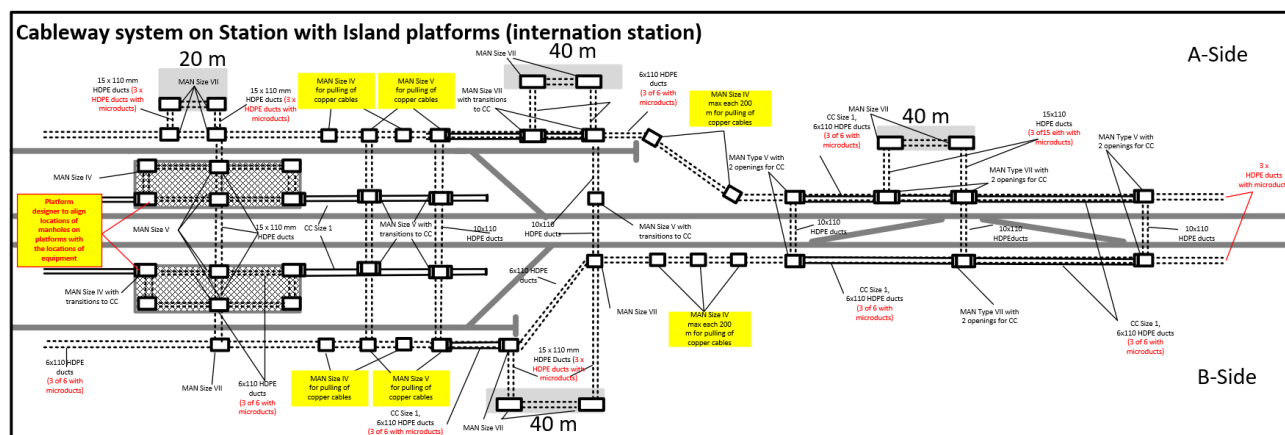
14. CABLEWAYS ON STATION WITH ISLAND PLATFORMS
