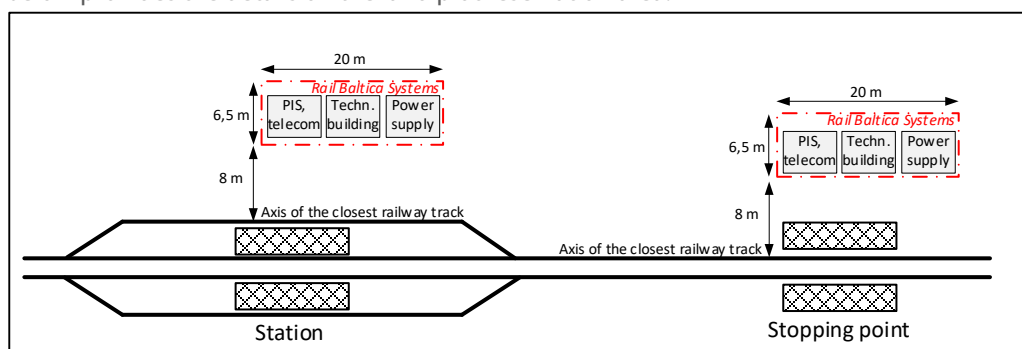
21. LAND PLOT RESERVATION AREA IN STATIONS AND STOPPING POINTS
