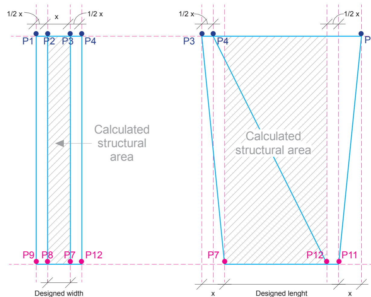
Elevations
