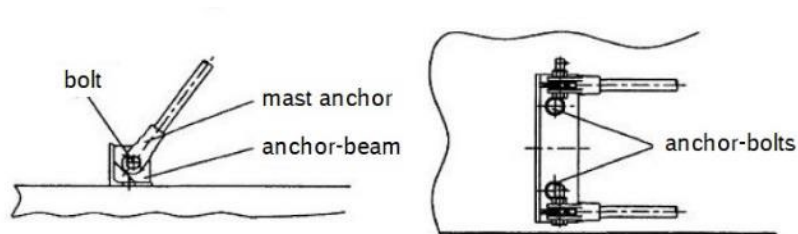
3. ANCHOR FOUNDATION
