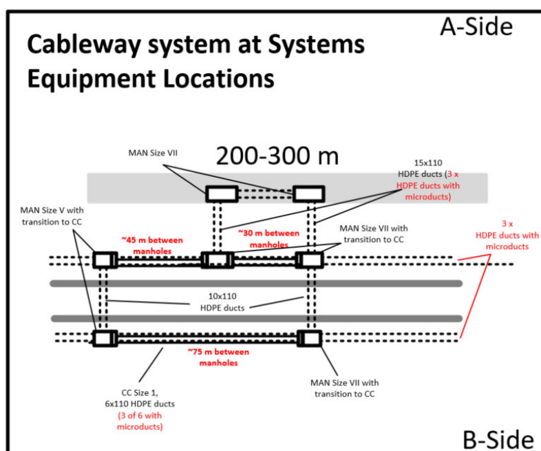
5. CABLEWAYS AT SYSTEM EQUIPMENT LOCATIONS
