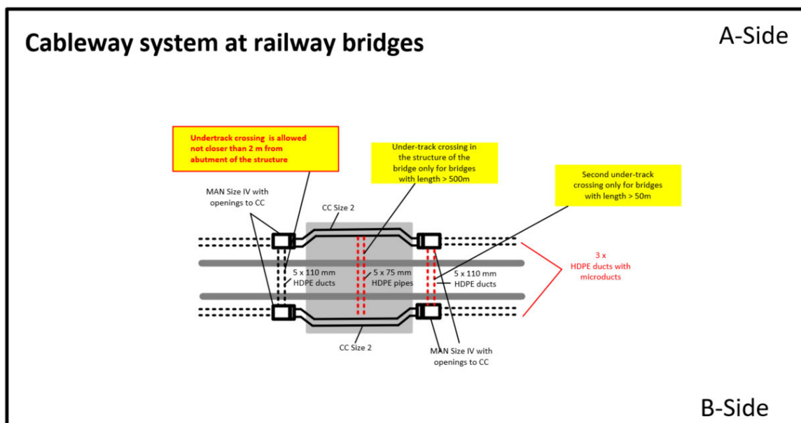
9. CABLEWAYS AT RAILWAY BRIDGES
