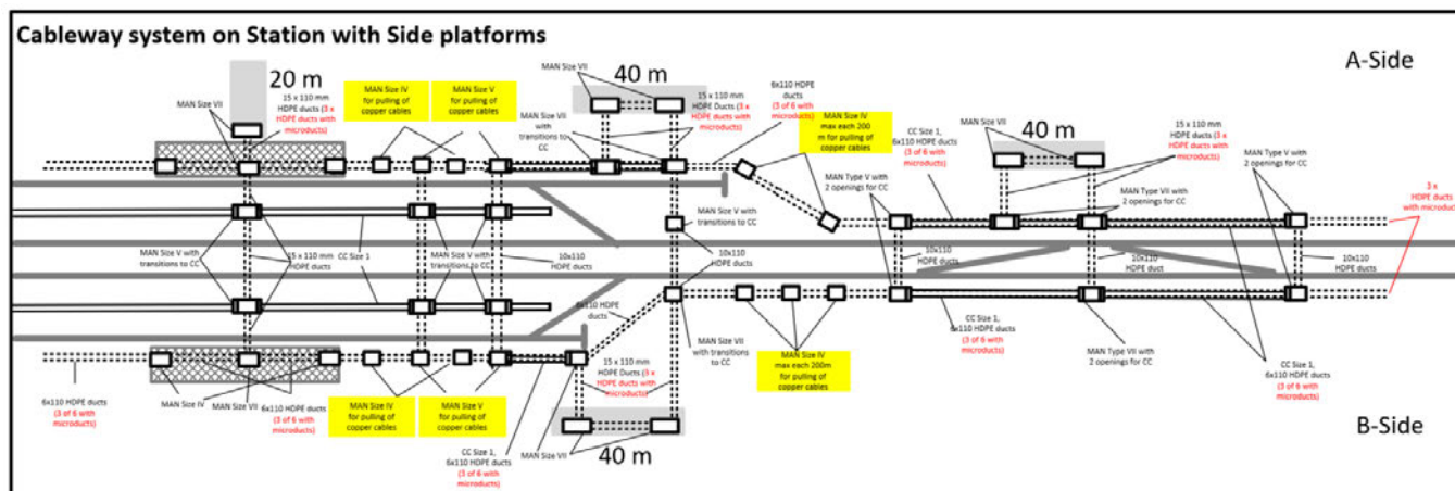
10. CABLEWAYS ON STATION WITH SIDE PLATFORMS
