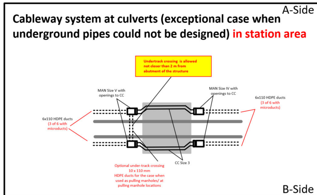
14. CABLEWAYS AT CULVERTS IN STATION AREA
