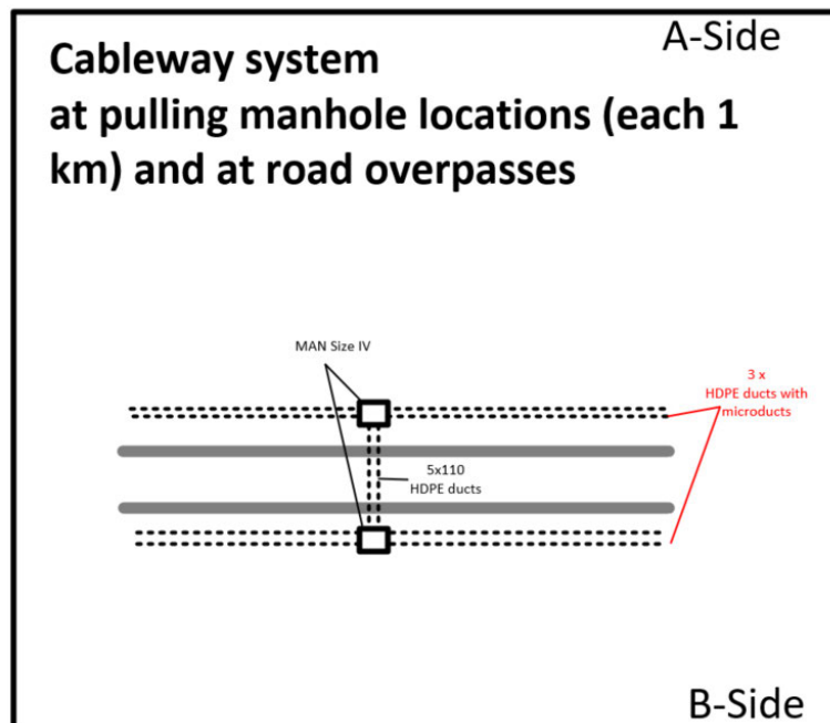
6. CABLEWAYS AT PULLING MANHOLES AND ROAD OVERPASSES
