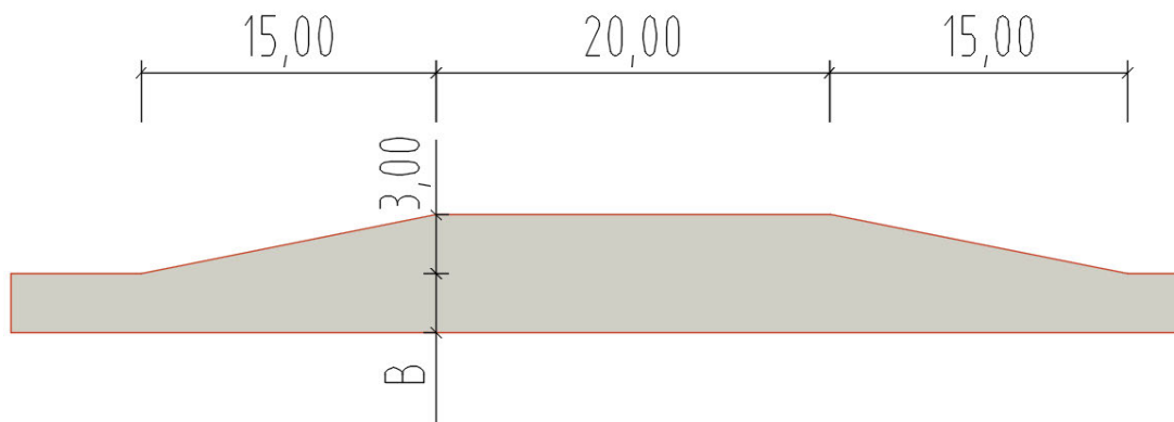
FIGURE 4 PASSING LOOP
