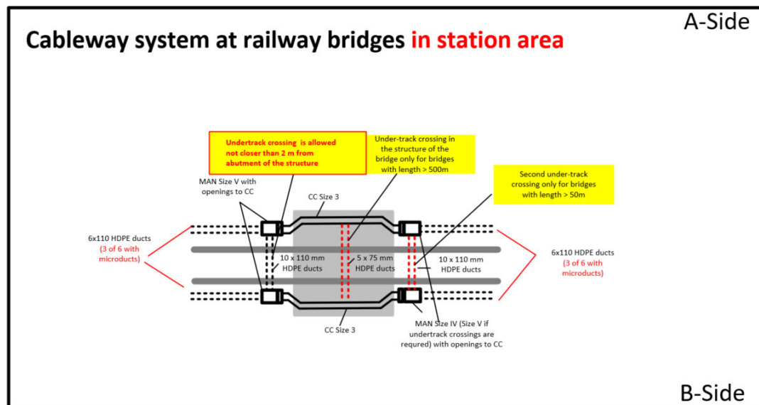
15. CABLEWAYS AT RAILWAY BRIDGES IN STATION AREA
