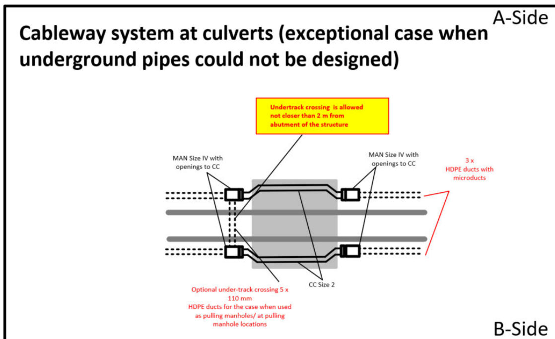
8. CABLEWAYS AT CULVERTS
