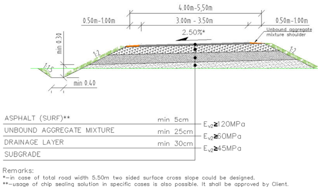
FIGURE 8 TYPICAL MAINTENANCE ROAD CROSS SECTION WITH BOUND MATERIAL SURFACE
