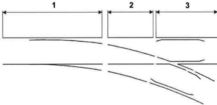
Figure 2, Turnout principle scheme
