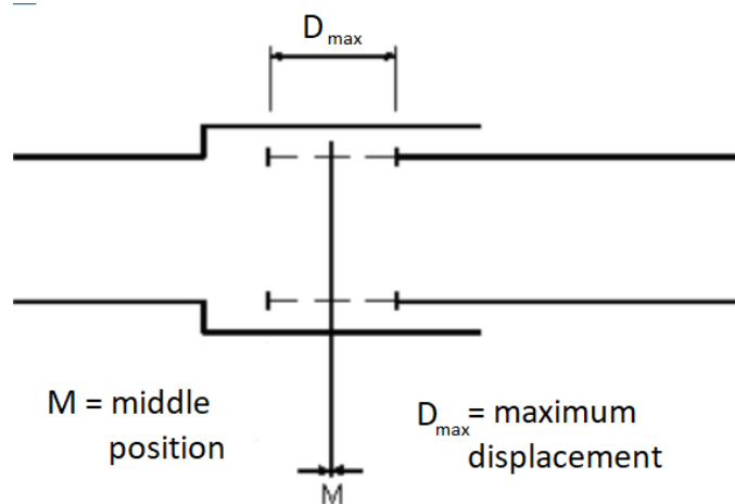
Figure 3, Rail expansion joint principal scheme
