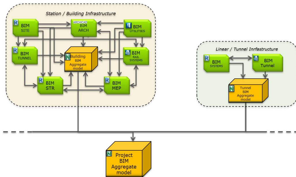
Figure 65: Example of aggregated model composition
