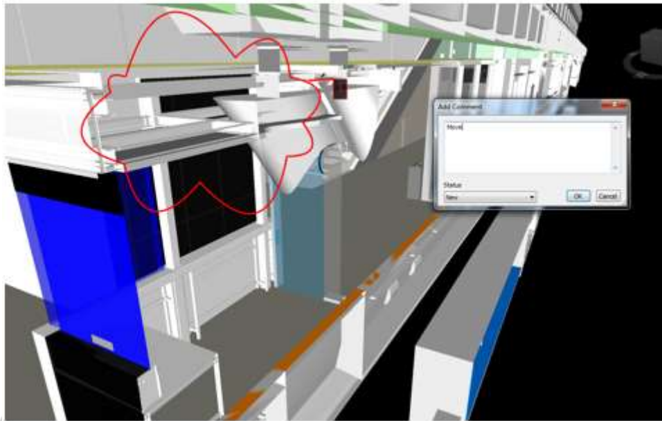
Figure 73: find of a clash during a Model Review
