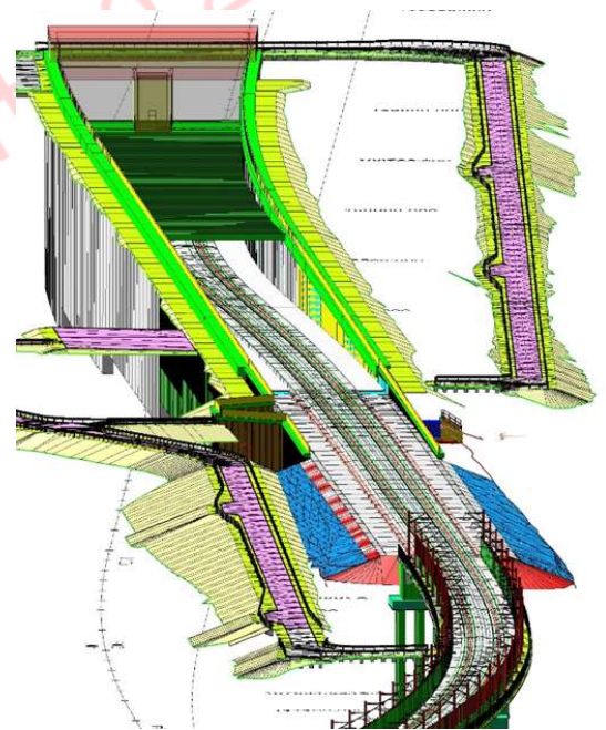
Figure 58: Example of linear infrastructure model
