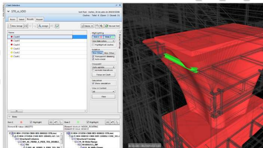
Figure 72: automatic interference checking software: Clash between Viaduct Structure and Station Structure
