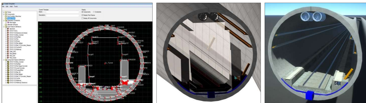
Figure 60: Example of tunnel model
