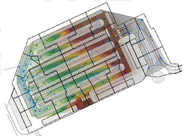
Figure 43: Example of drainage model
