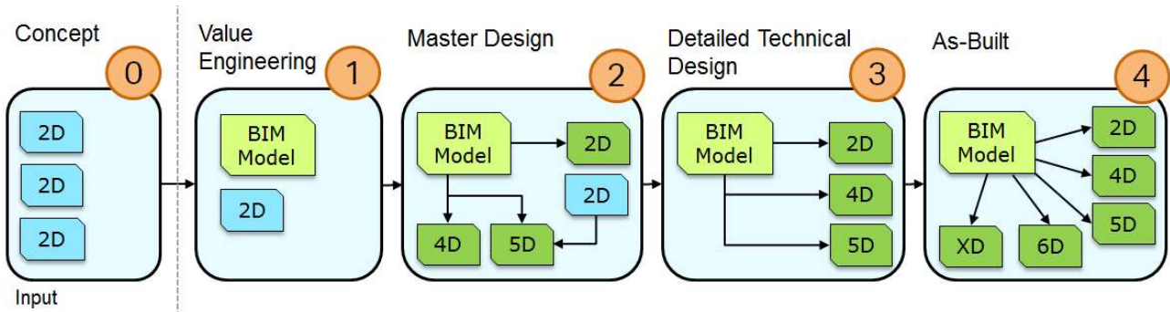
Figure 5: Steps from 2D to As-Built BIM Model
