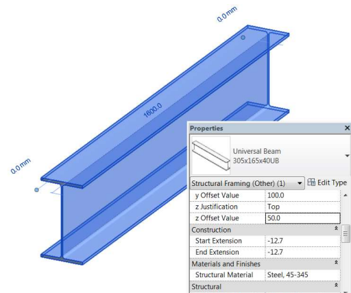
Figure 49: Example of BIM Object geometry and information attached
