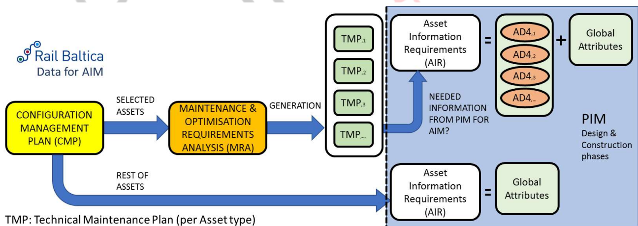
Figure 34: Requirements development
